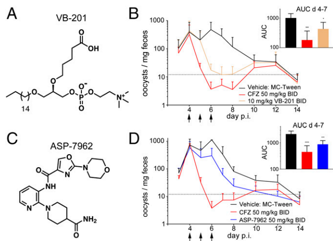
Fig. 3. ReFRAME library compounds with anticryptosporidial efficacy. (A and C) The structures of oxidized phospholipid VB-201 and TrkA inhibitor ASP-7962. ASP-7962 is a best-guess structure from a phase 2 trial. (B and D) Oocyst shedding trace of mice infected with 1 \times 10^6 oocysts on day 0, then monitored for 2 wk. Line graph data are weight-adjusted mean oocyst counts \pm SD ( n = 8 over two separate experiments). (B and D, Insets ) Bar graphs are oocyst counts \pm SEM ( n = 4 ) measured on day 7. These data were assessed with one-way ANOVA. Treatments were compared with the previously investigated compound clofazimine (CFZ) (50 mg/kg BID). AUC, area under the curve. * P < 0.05 ; *** P < 0.005 ; **** P < 0.001 .
